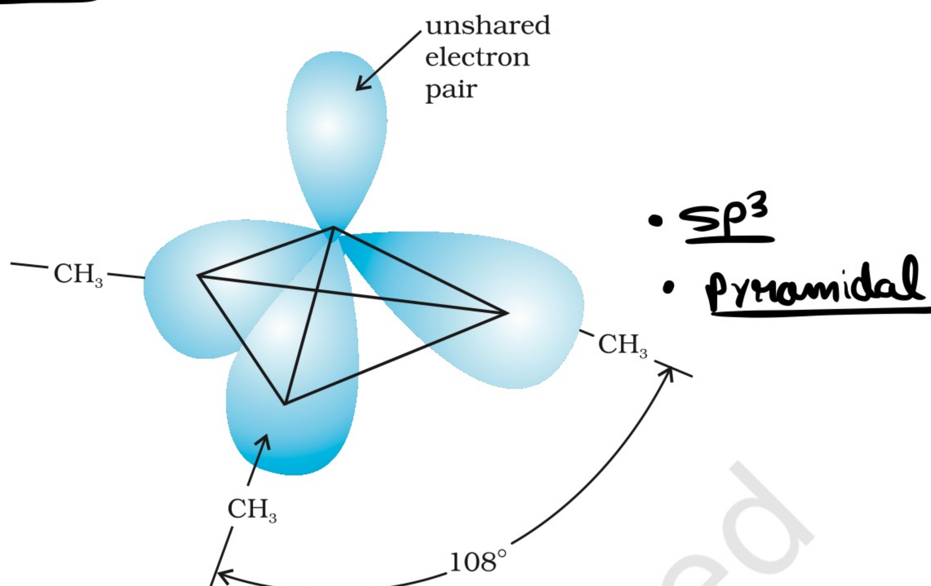
Fig. 13.1 Pyramidal shape of trimethylamine
