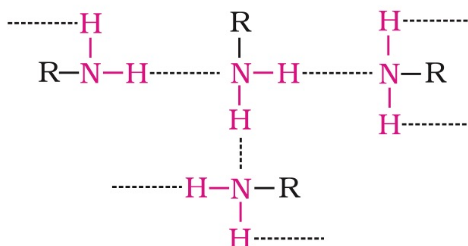
Fig. 13.2 Intermolecular hydrogen bonding in primary amines
